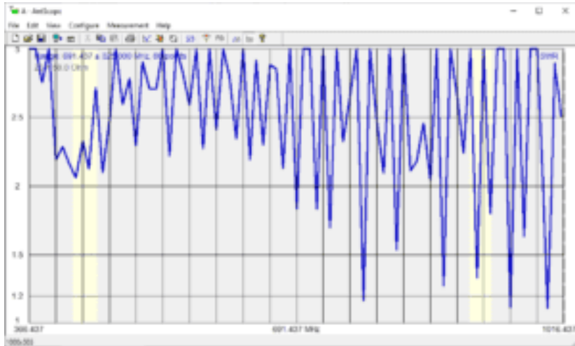
366.437 to 1016.437 MHz SWR Analysis
