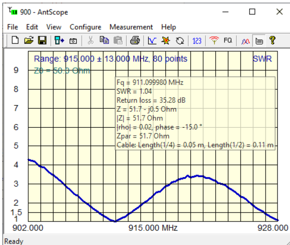
900 MHz Meter SWR Analysis
